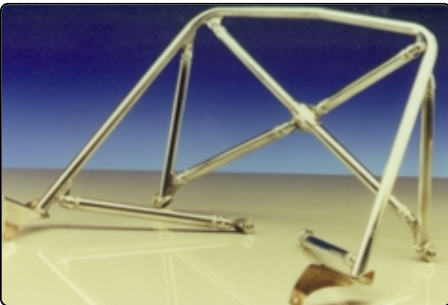
Safety roll bar RS with cross strut bars
